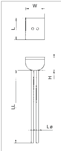
Picture applies to sensor: L 220 P Pt 100
