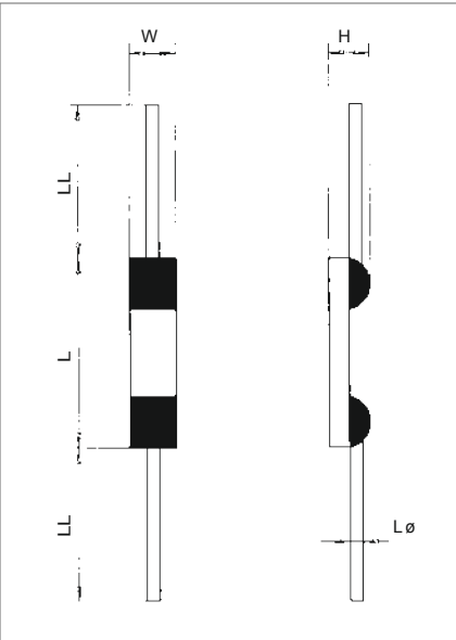
Pictures applies to (ax) M-sensor types. The measuring point for the basic value is situated at 8 mm from the end of the sensor body.
